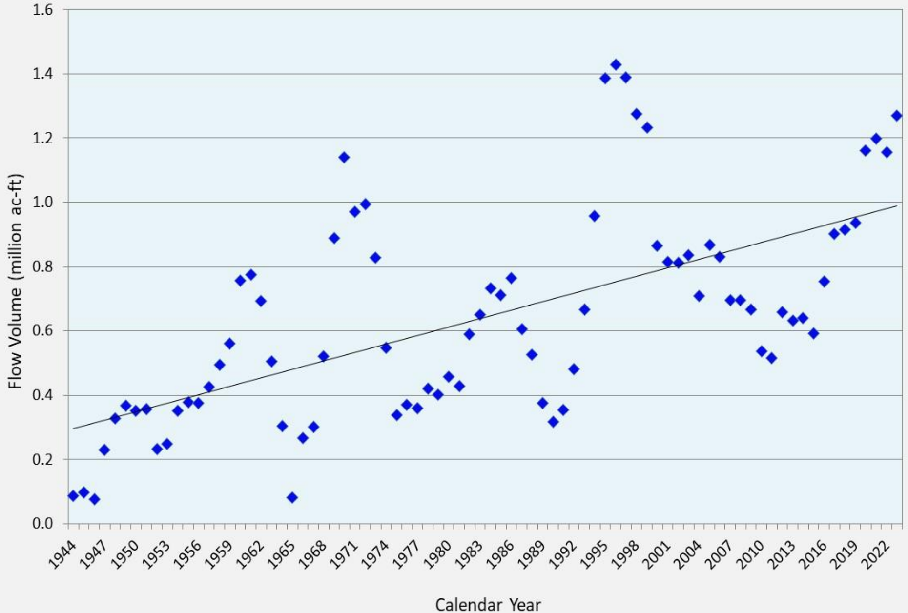
5-Year Average Flow to Everglades National Park at Tamiami Trail Each data point is the computed average for the five years ending with that year
