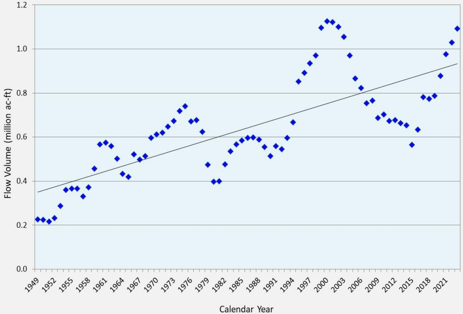
10-Year Average Flow to Everglades National Park at Tamiami Trail Each data point is the computed average for the ten years ending with that year
