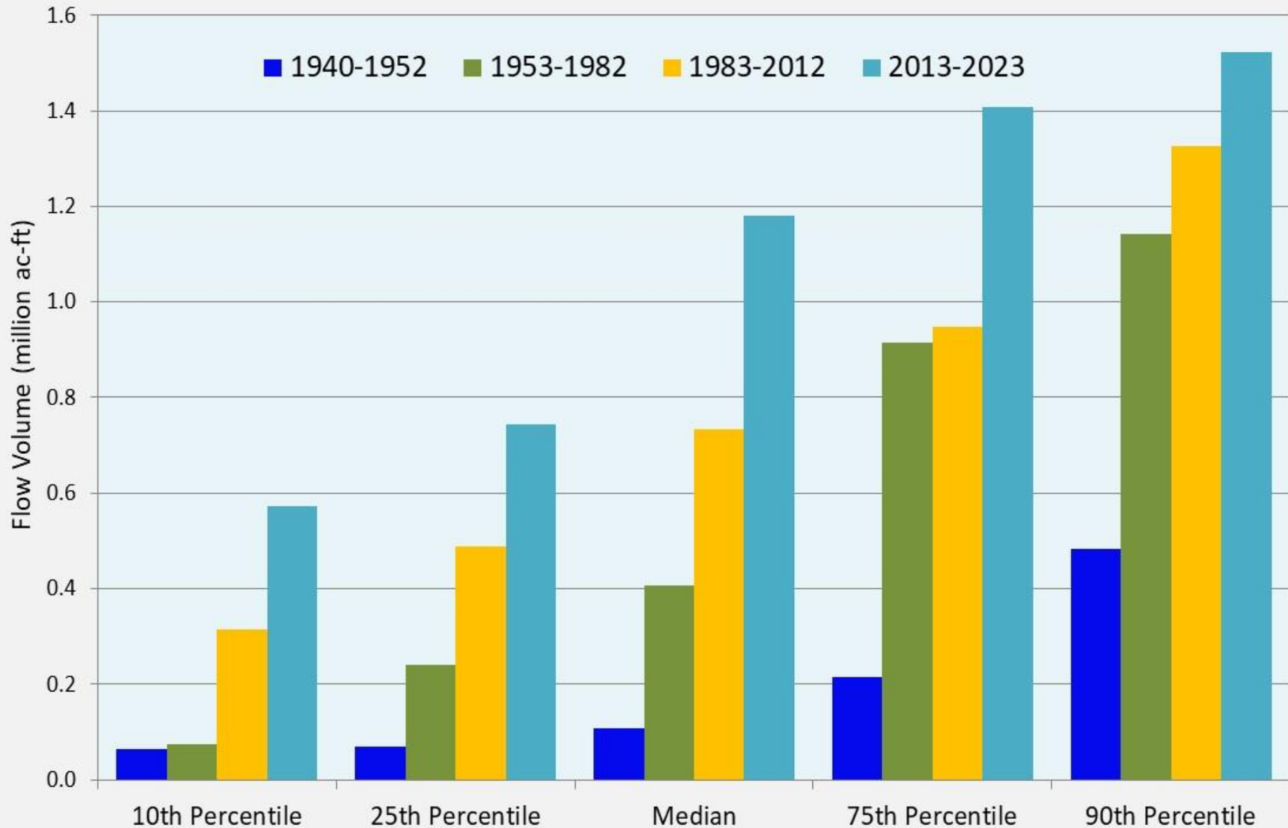
Frequency Distribution of Annual Flow to Everglades National Park at Tamiami Trail Sum of S-12A-D, S-333, S-333N, S-356 and S-355A-B
