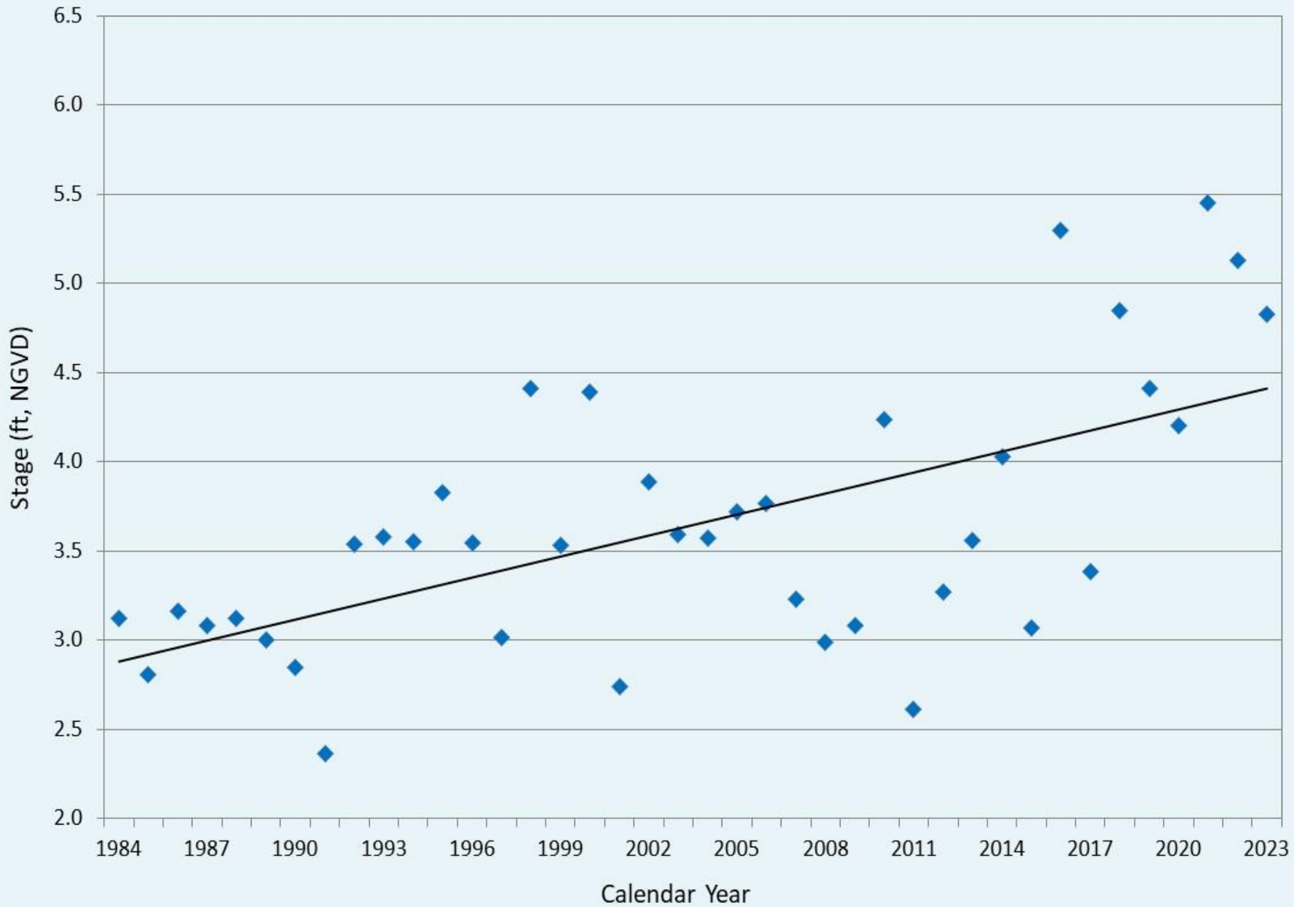
Average Dry Season (January-April) Stage at Northern Taylor Slough Since 1984 (DBKEY: 6724)
