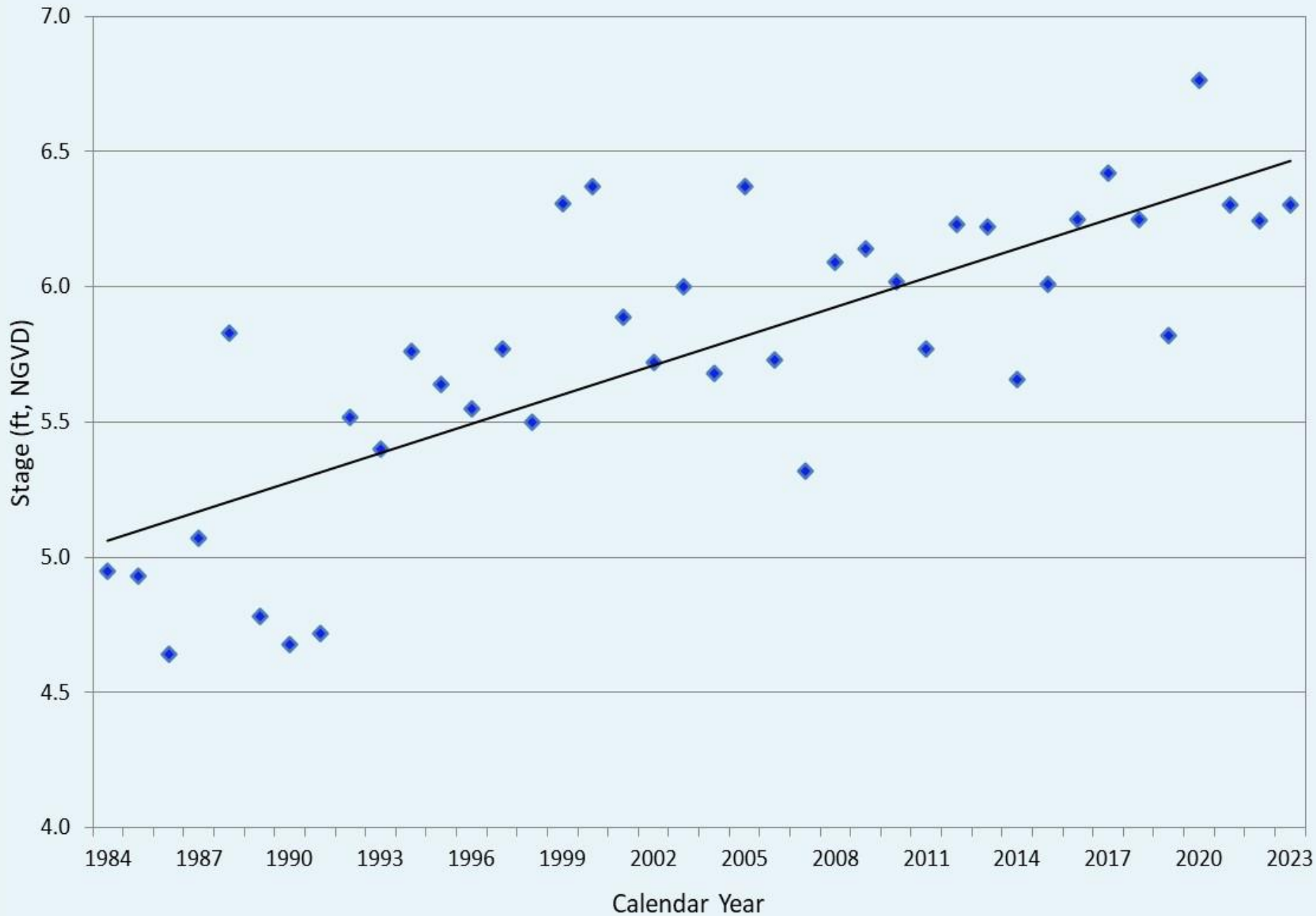
Maximum Annual Stage at Northern Taylor Slough Since 1984 (DBKEY: 6724)
